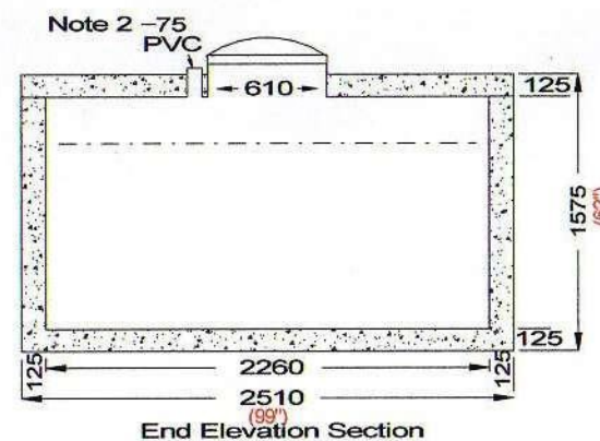
End Elevation Section
