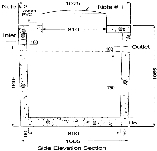
Side Elevation Section
