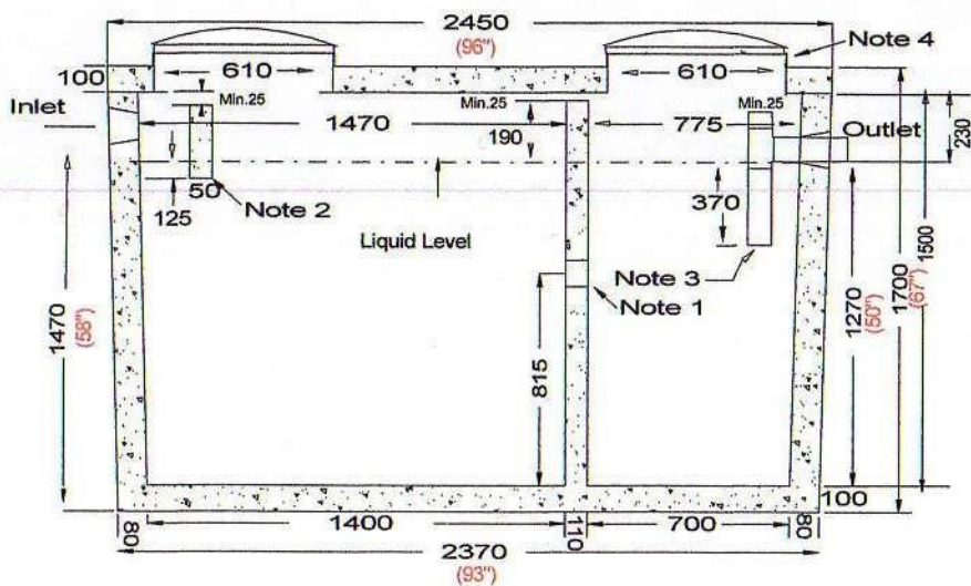
Side Elevation Section
