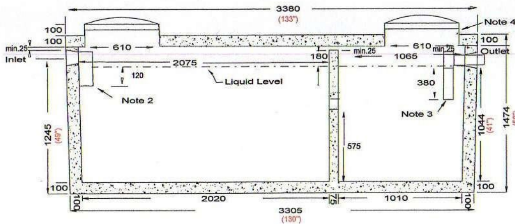
Side Elevation Section
