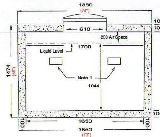
End Elevation Section
