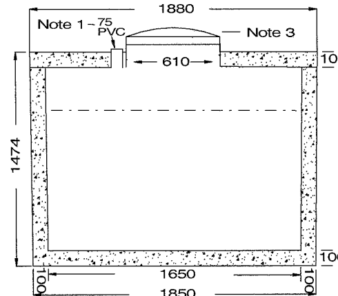
End Elevation Section
